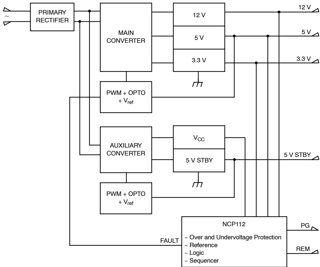
Figure 3. Simplified Application Schematic
