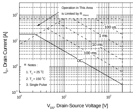
Figure 9-2. Maximum Safe Operating Area for FQPF18N20V2
