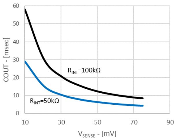
COU Period vs V_{SENSE}
