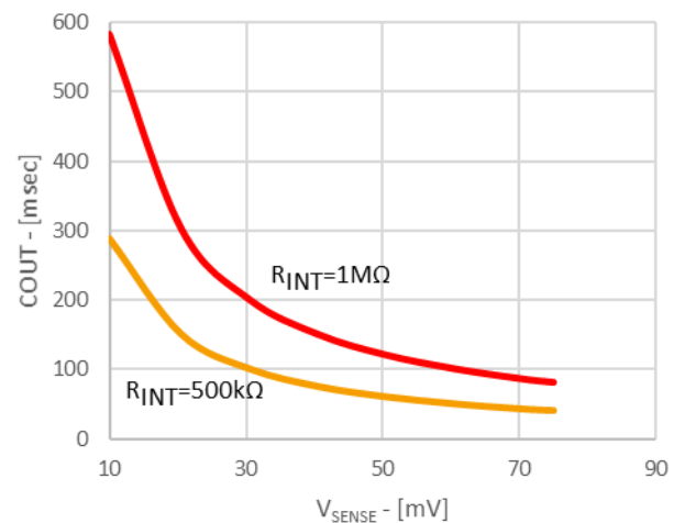
COU Period vs V_{SENSE}
