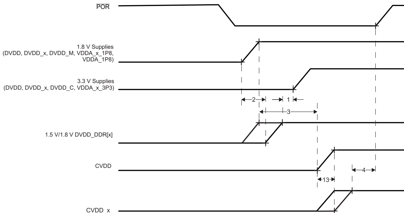
Figure 7-1. Power-Up Sequence
