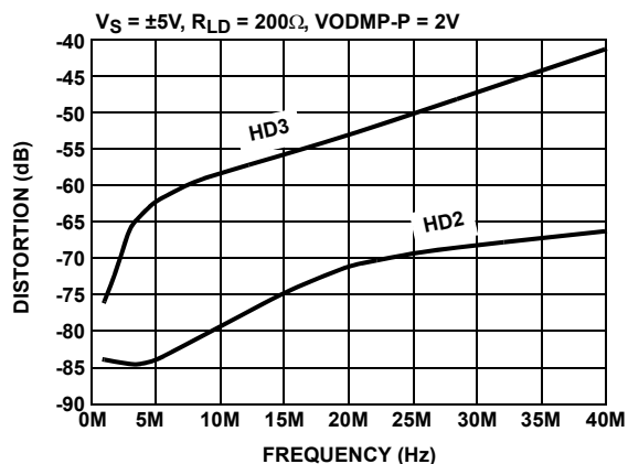
FIGURE 16. HARMONIC DISTORTION vs FREQUENCY
