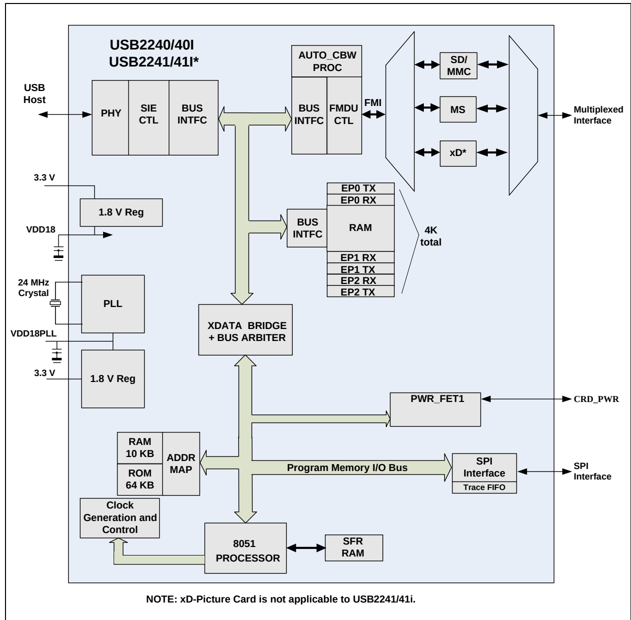
FIGURE 3-1: USB2240/40I/41I/41I* BLOCK DIAGRAM
