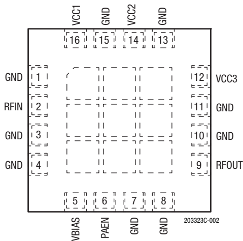
Figure 2. SKY66297-11 Pinout (Top View)
