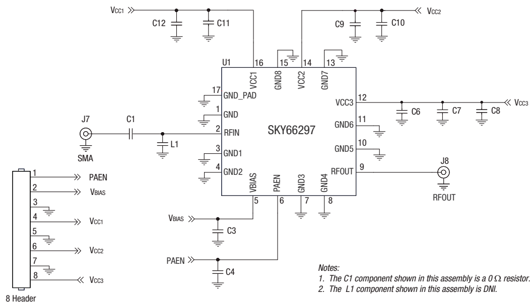
Figure 17. SKY66297-11 Evaluation Board Schematic
