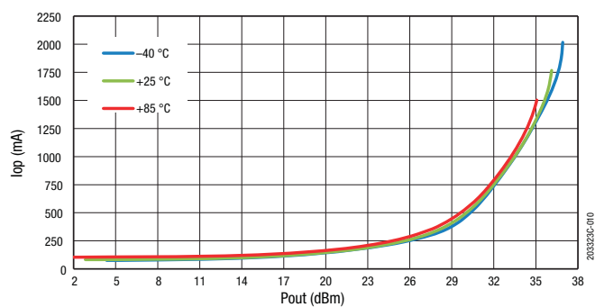
Figure 10. Operating Current vs Pout Across Temperature (CW)
