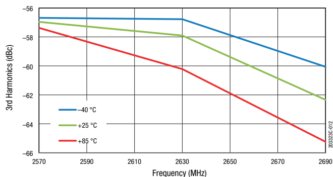
Figure 12. 3rd Harmonic vs Frequency @ POUT = +28 dBm (CW) Across Temperature
