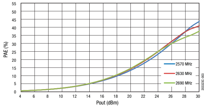
Figure 3. PAE vs Pout Across Frequency (CW)
