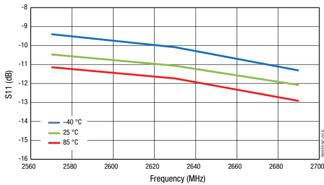
Figure 15. Input Return Loss vs Frequency Across Temperature ( P_{IN} = -20 dBm)
