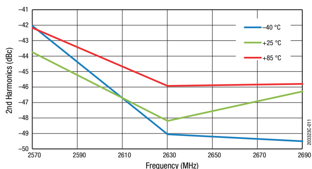
Figure 11. 2nd Harmonic vs Frequency @ POUT = +28 dBm (CW) Across Temperature
