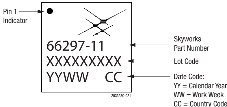
Figure 21. Typical Part Marking for the SKY66297-11
