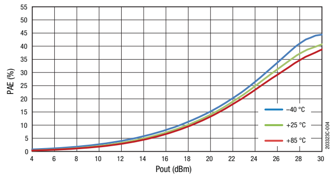
Figure 4. PAE vs Pout Across Temperature (CW)
