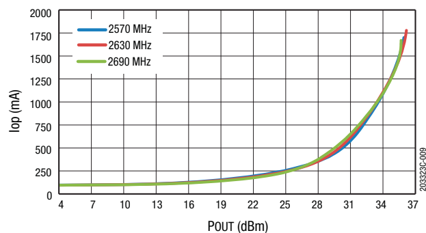
Figure 9. Operating Current vs Pout Across Frequency (CW)
