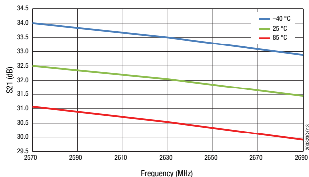
Figure 13. Small Signal Gain vs Frequency Across Temperature (PIN = -30 dBm)
