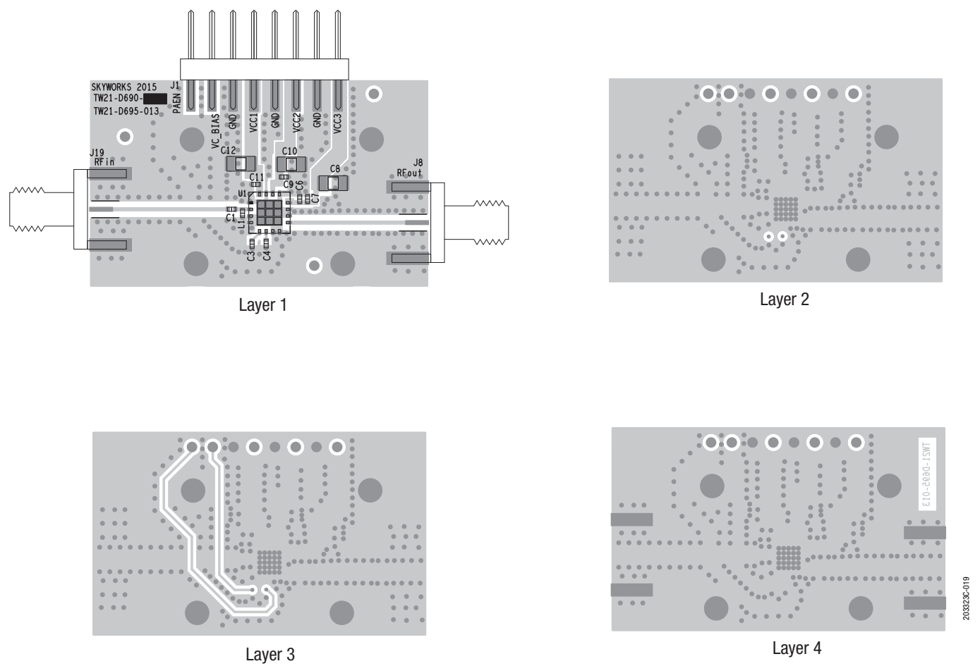
Figure 19. Evaluation Board Layer Details
