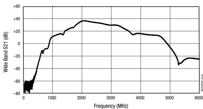
Figure 14. Wide Band Small Signal Gain vs Frequency (PIN = -30 dBm)
