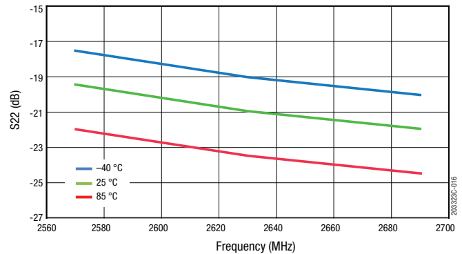
Figure 16. Output Return Loss vs Frequency Across Temperature ( P_{IN} = -20 dBm)
