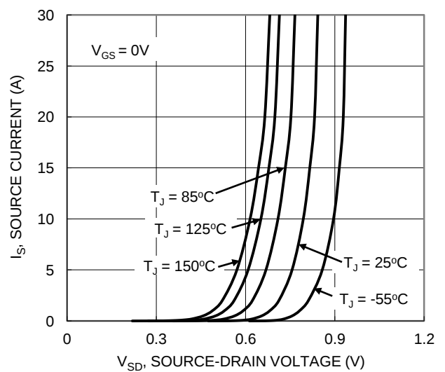
Figure 18. Q2 Diode Forward Voltage vs. Current
