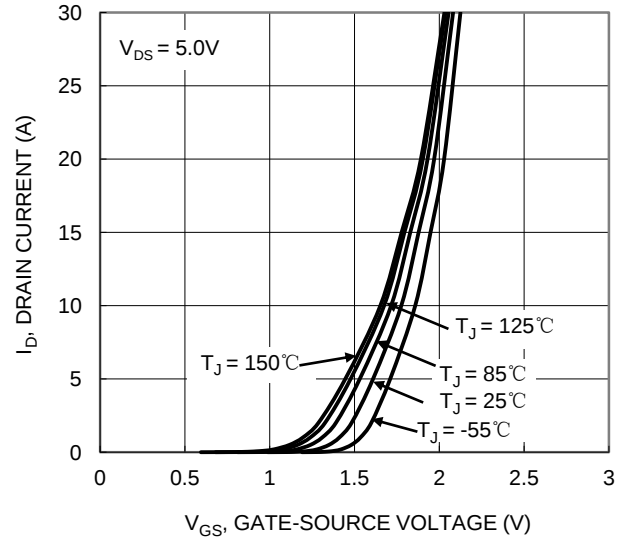
Figure 4. Q2 Typical Transfer Characteristic
