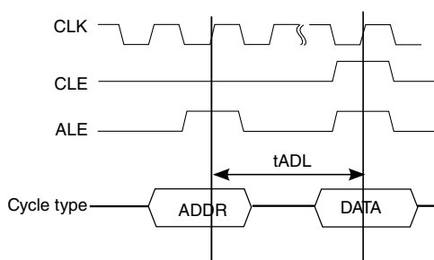
Figure 51. t_{ADL} timings
