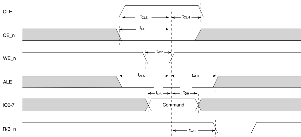
Figure 34. Command cycle
