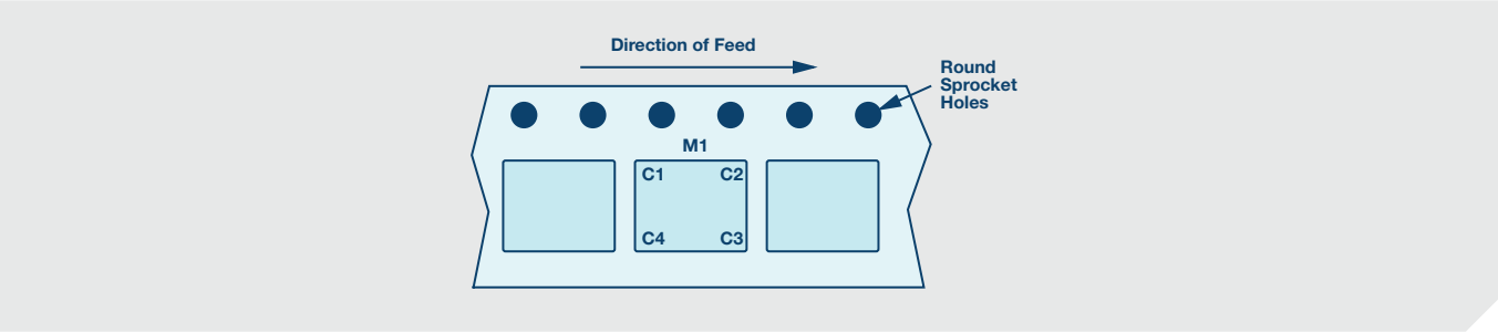
Figure 2. Pin 1 orientation reference.
