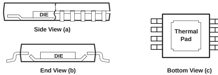
Figure 46. Views of Thermally Enhanced DGN Package
