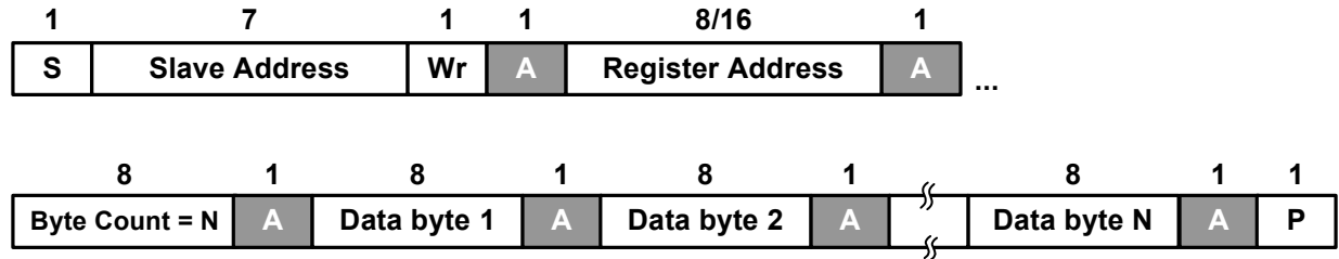
Figure 5.12 Block Write
