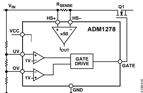
Figure 57. Undervoltage and Overvoltage Supply Monitoring
