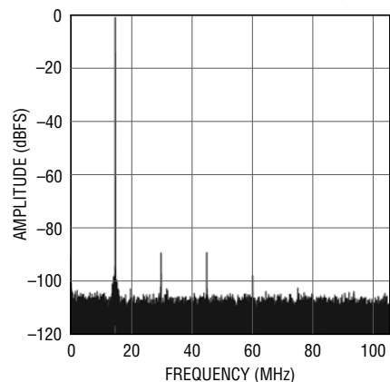
LTC2156-14: 32K Point FFT, f_{IN} = 15\text{MHz} , -1\text{dBFS} , 210MSPS
