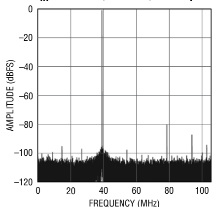
LTC2156-14: 32K Point FFT, f_{IN} = 171\text{MHz} , -1\text{dBFS} , 210MSPS
