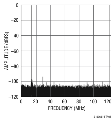
LTC2157-14 32K Point FFT, f_{\text{IN}} = 15\text{MHz} , -1\text{dBFS} , 250Msps
