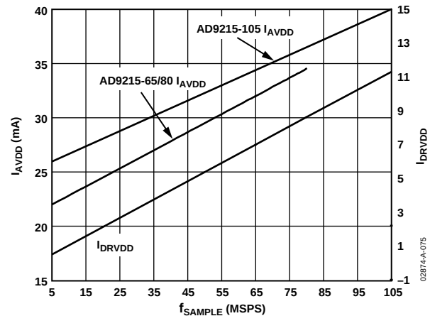
Figure 35. Supply Current vs. f_{\text{SAMPLE}} for f_{\text{IN}} = 10.3 MHz
