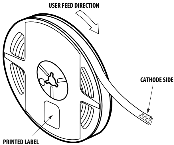
Figure 20. Reeling Orientation
