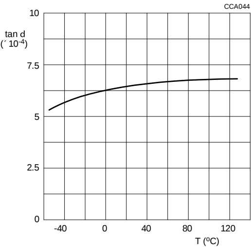
Fig. 8 Typical \tan \delta as a function of temperature
