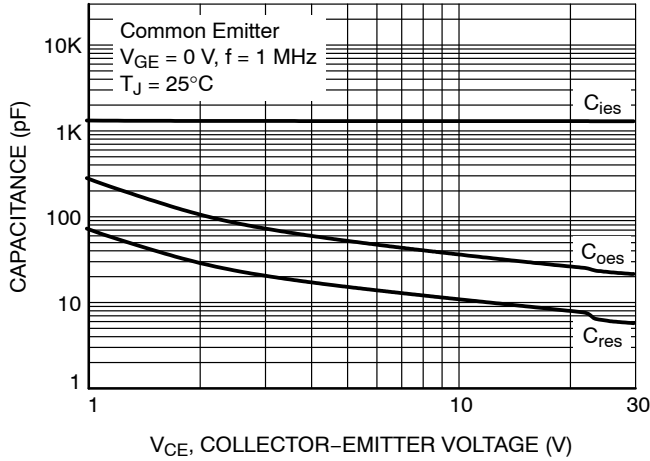
Figure 7. Capacitance Characteristics
