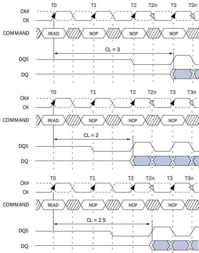
Figure 6: CAS Latency Diagram
