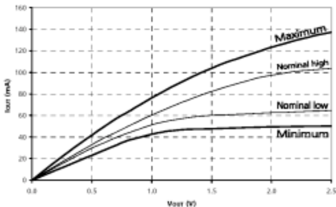
Figure 8: Pull-Down Characteristics
