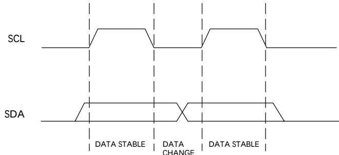
Figure 12: Data Validity
