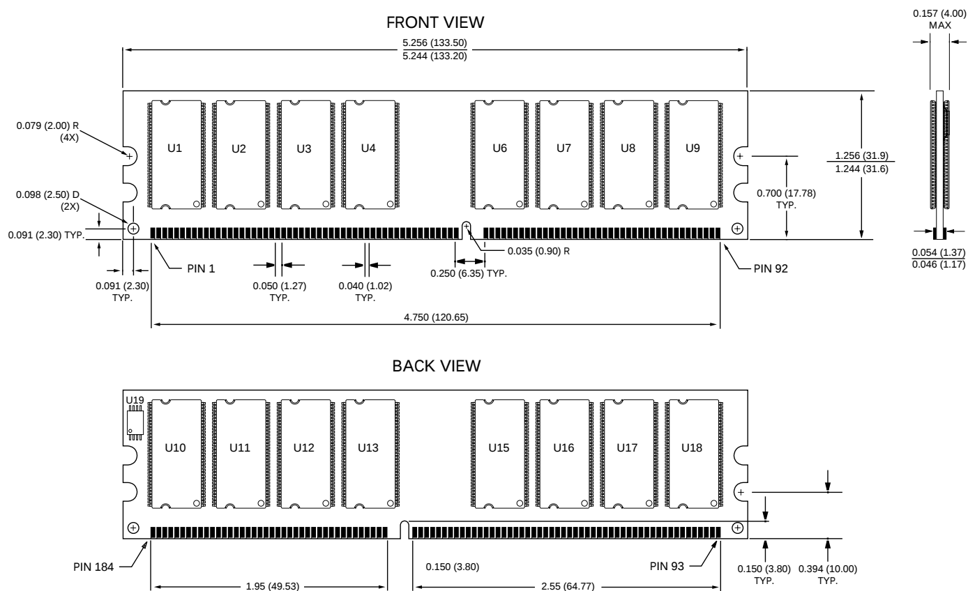
Figure 16: 184-PIN DDR DIMM Dimensions – Standard PCB
