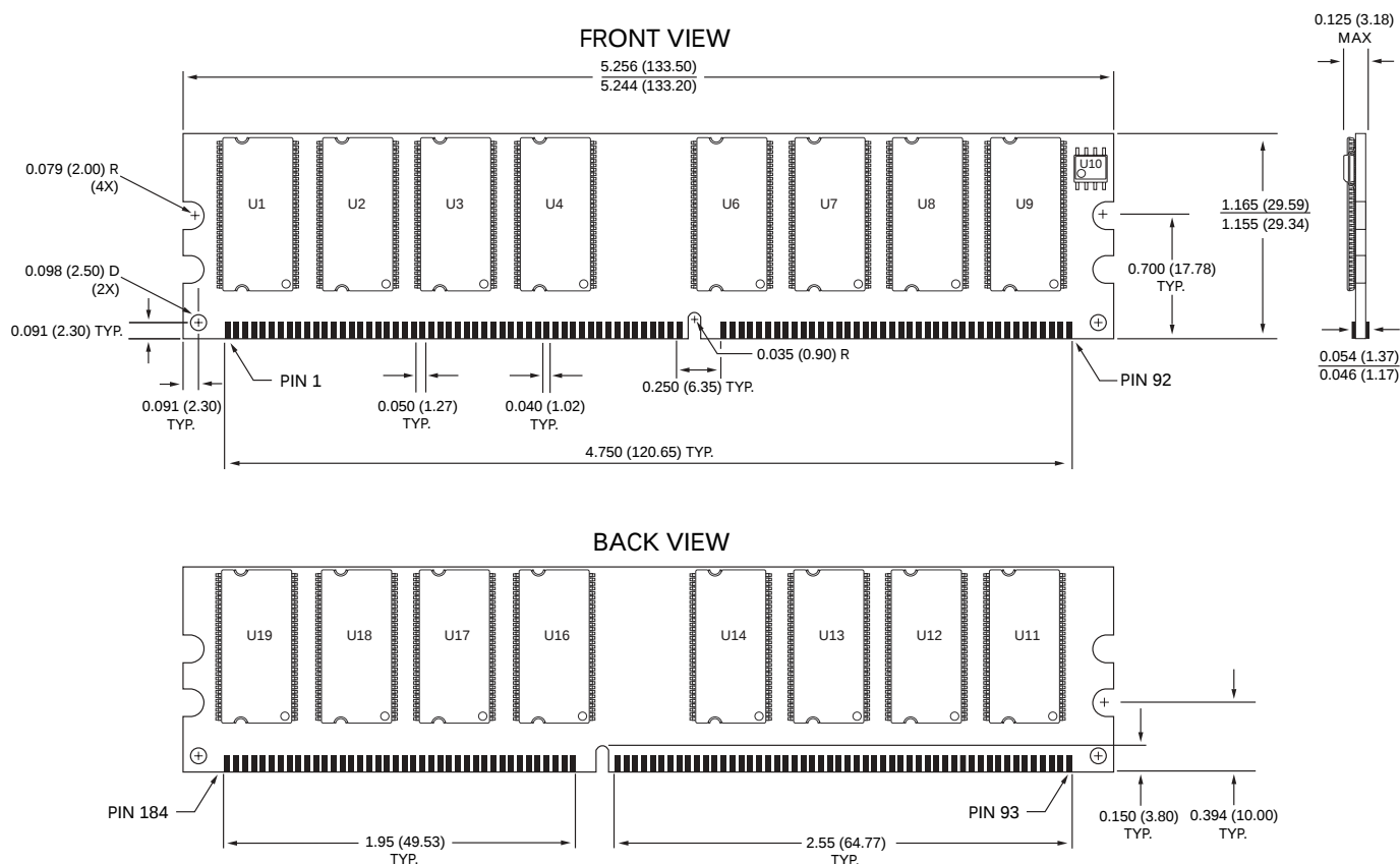
Figure 17: 184-PIN DDR DIMM Dimensions – Low-Profile PCB
