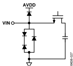
Figure 34. Equivalent Analog Input Circuit
