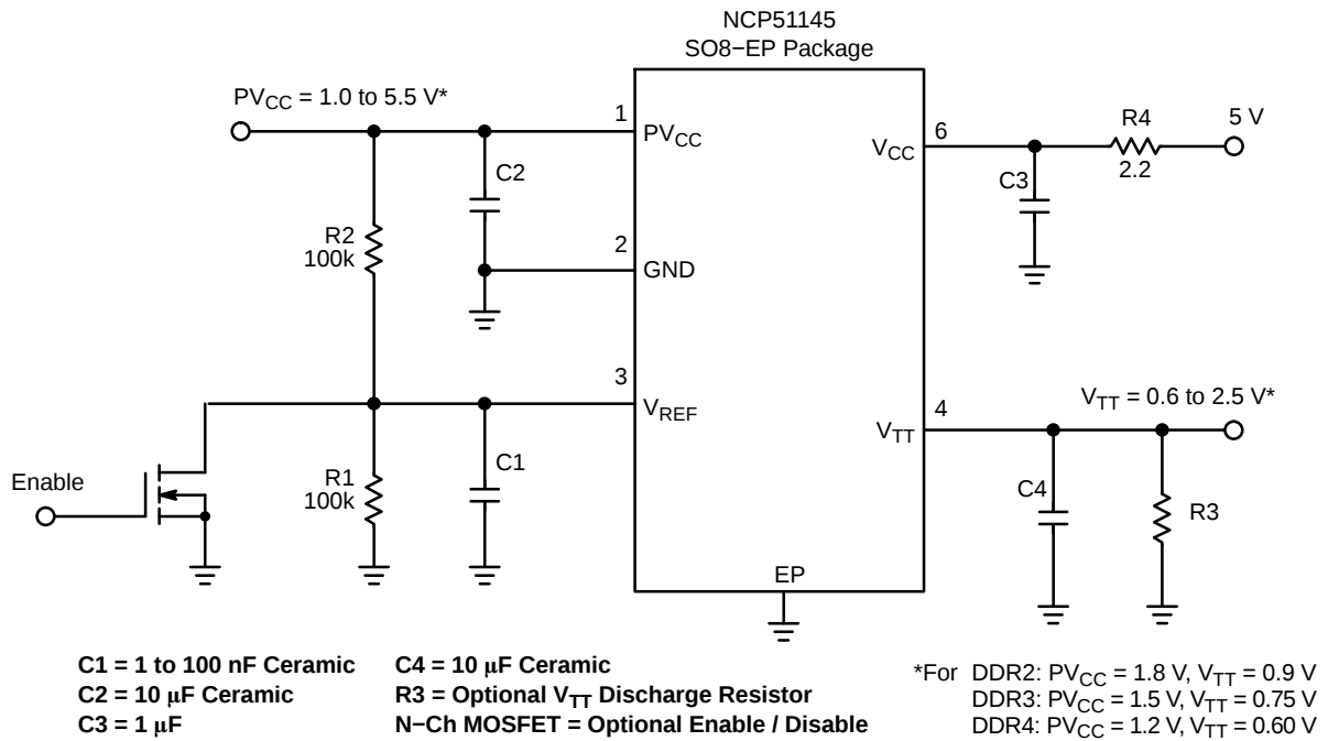
Figure 1. Application Diagram
