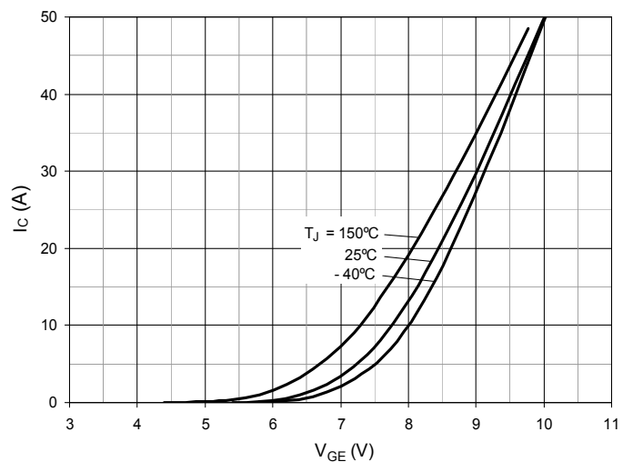
Fig. 6. Input Admittance
