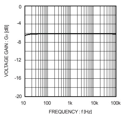
Fig.8 Voltage gain vs Frequency (BD3824FS)
