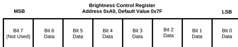
Figure 46. Brightness Control Register
