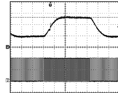
Channel 2: PWM (5V/div) Channel 4: I_{LED} (5mA/div) D_{PWM} From 30% To 70% F_{PWM} = 5\text{ kHz} Time Base (2ms/div) I_{LED} Full Scale = 19 mA
