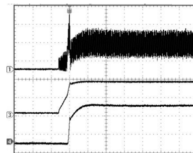
Channel 1: I_{IN} (200mA/div) Channel 3: V_{OUT} (20V/div) Channel 4 ( I_{LED} ) (10mA/div) L = 22\text{ }\mu\text{H} V_{IN} = 3.6\text{ V} Time Base (2ms/div) Ramp Rate = 8μs/Step I_{LED} = 19\text{ mA}
