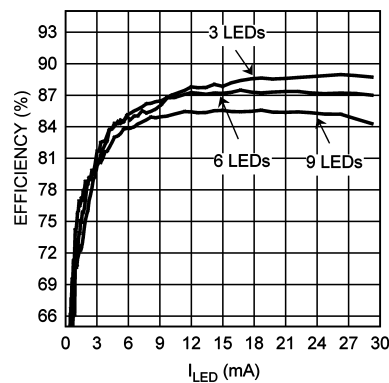
Figure 53. Efficiency vs I_{\text{LED}}
