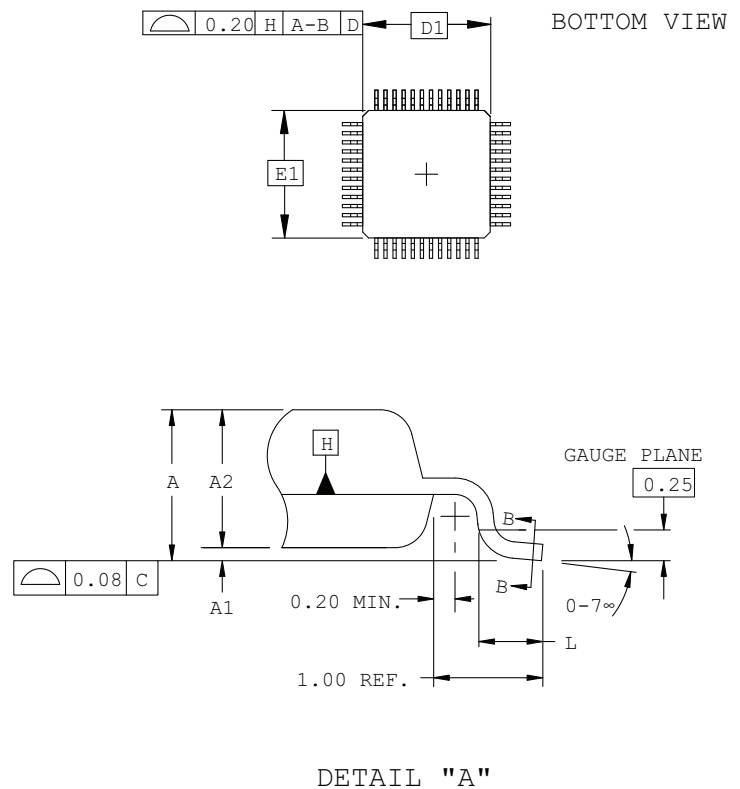
DETAIL "A"
