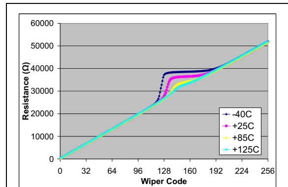
FIGURE 2-54: 50 kΩ – R_{WB} (Ω) vs. Wiper Setting and Ambient Temperature ( V_{DD} = 3.0\text{V} , I_W = 48\text{ }\mu\text{A} ).
