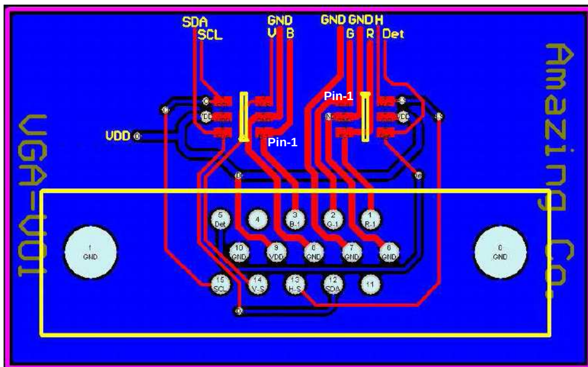
Fig. 6 The PCB layout example for a VGA port with two AZC399-04S being used.
