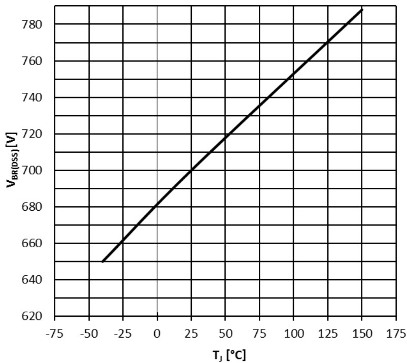
Figure 27 Drain-source breakdown voltage ICE5xRxx70AG; V_{BR(DSS)}=f(T_J) , I_D=1 mA
