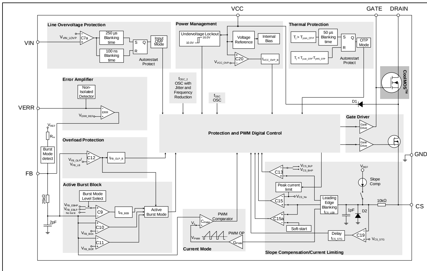
Figure 4 Representative block diagram
