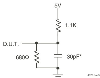
Figure 2. Output Load
