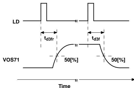
Figure 10. t_{d3r} and t_{d3f} Measurement References
