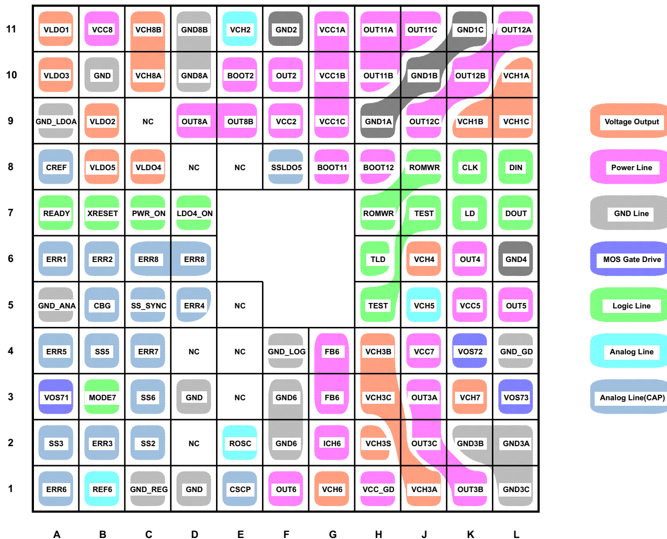
Figure 15. Pin Layout
