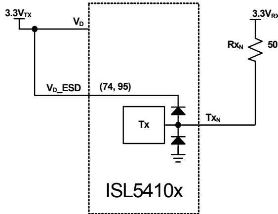
FIGURE 10. ISL5410x ESD PROTECTION DIODES
