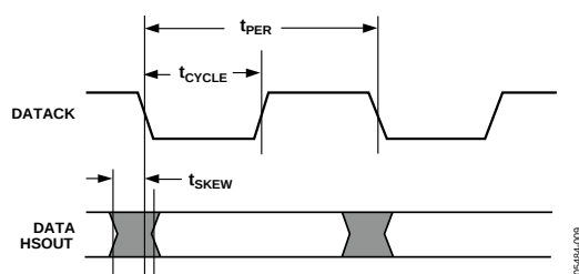
Figure 9. Output Timing
