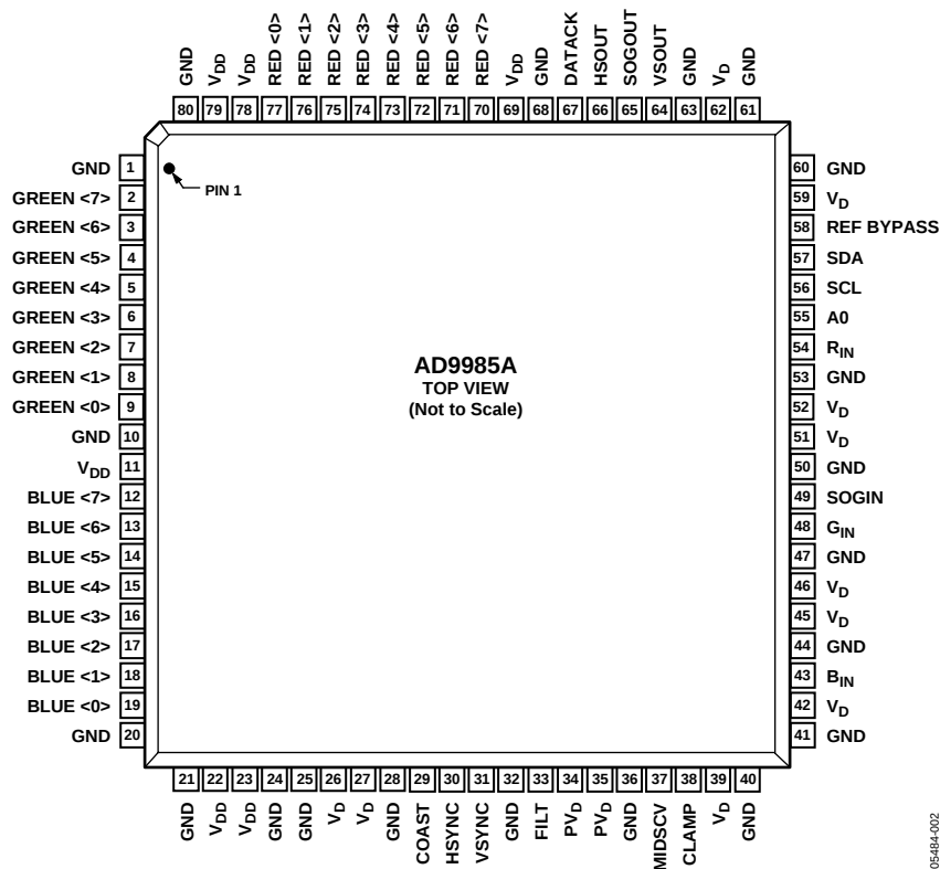
Figure 2. Pin Configuration
