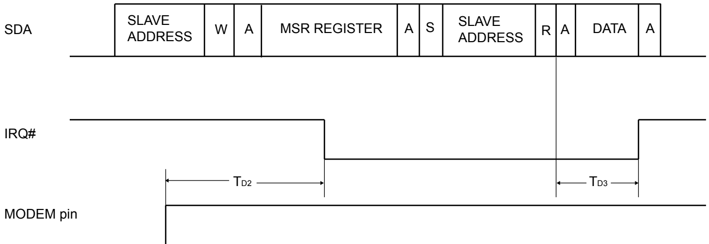
Figure 4. Modem Input Pin Interrupt
