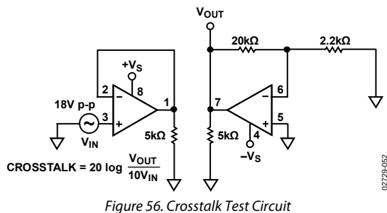
Figure 56. Crosstalk Test Circuit
