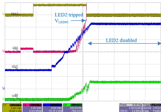
Figure 36: A80601 startup sequence when LED string#2 has a partial-short fault (6 × WLED instead of 8). As soon as LED2 pin rises above V_{LEDSD} (~5 V), the channel is disabled and FAULT = Low.
