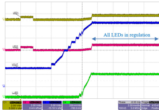
Figure 35: A80601 Normal startup sequence showing voltage at LED1 and LED2 pins. V_{IN} = 6 V, output = 8 × WLED in series, current = 4 × 100 mA
