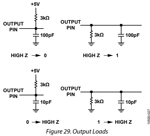
Figure 29. Output Loads
