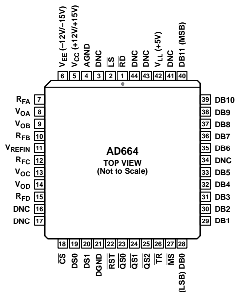
Figure 4. 44-Lead PLCC Pin Configuration
