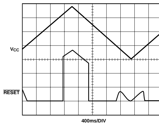
Figure 8. ADM706/ADM708 \overline{\text{RESET}} Output Voltage vs. Supply Voltage
