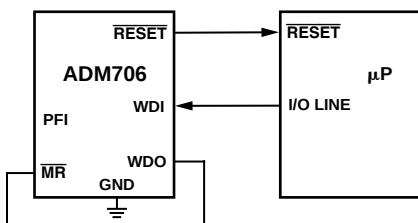
Figure 16. \overline{\text{RESET}} from WDO
