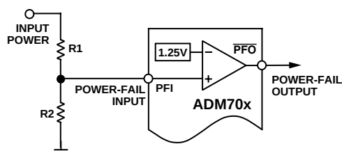
Figure 5. Power-Fail Comparator
