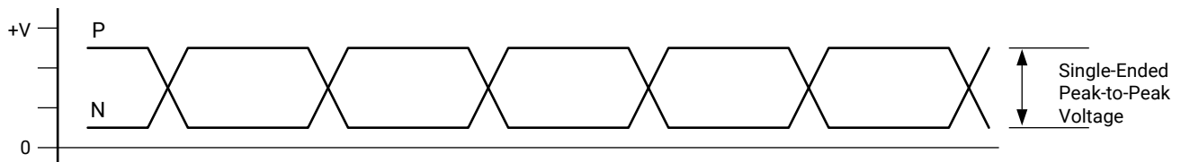
Figure 5: Single-Ended Peak-to-Peak Voltage
