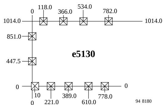
Figure 5. Pad coordinates
