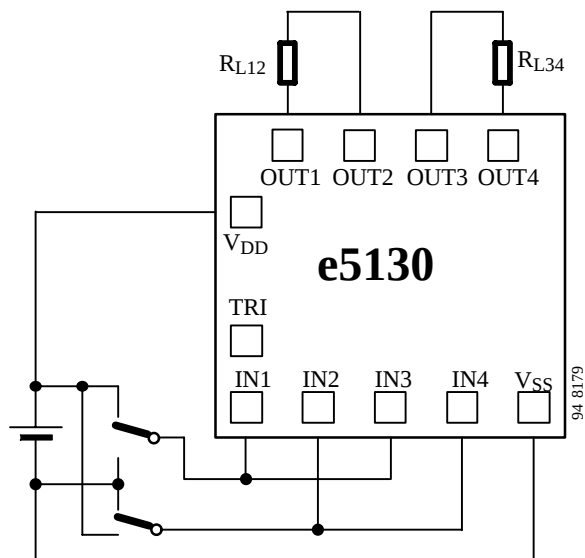
Figure 1. Test circuit
