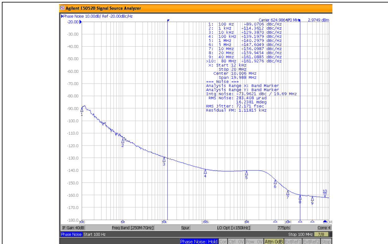
FIGURE 7-4: 625.0000 MHz, Integration Range 12 kHz to 20 MHz: 72.1 f_{\text{RMS}} .
