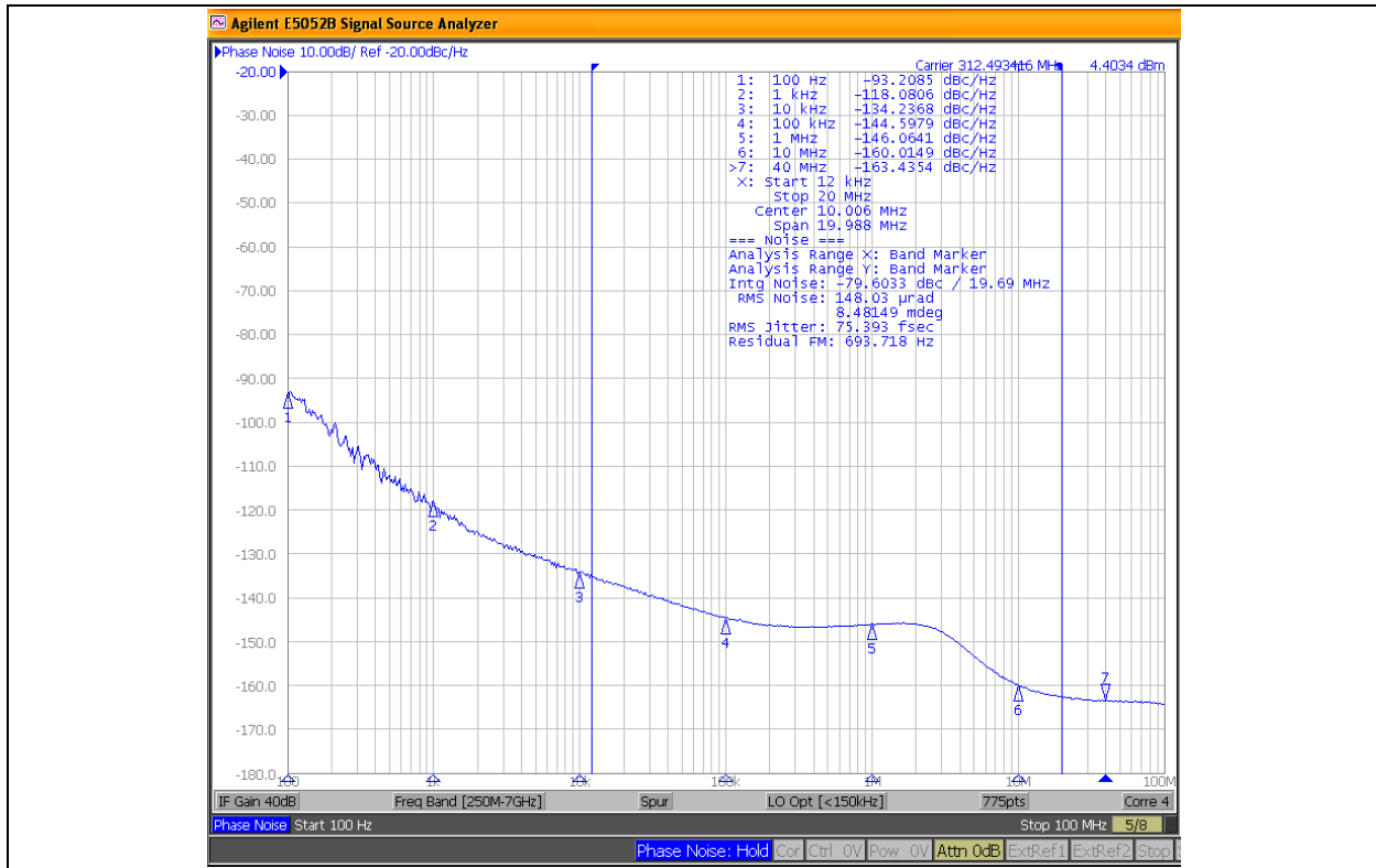
FIGURE 7-3: 312.500 MHz, Integration Range 12 kHz to 20 MHz: 75.4 f_{\text{RMS}} .
