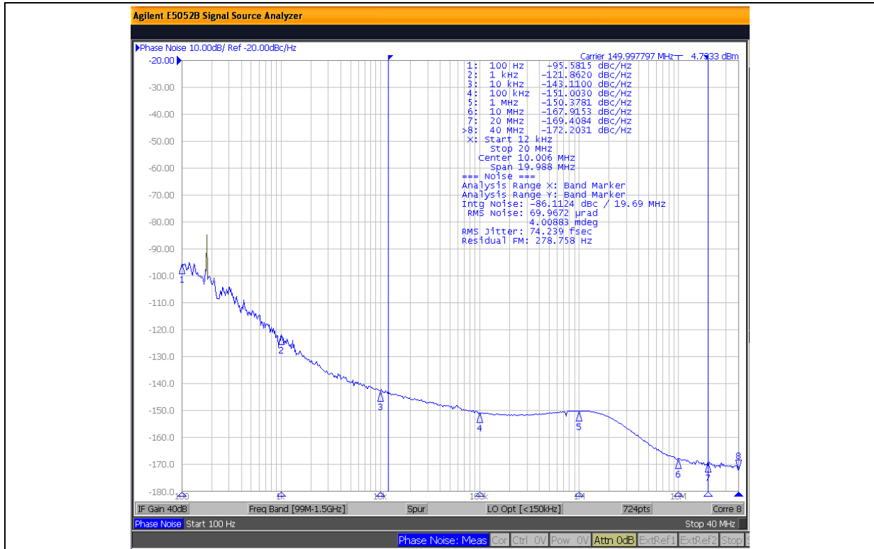
FIGURE 7-1: 150.0000 MHz, HCSL, Integration Range 12 kHz to 20 MHz: 74.2 fs RMS .
