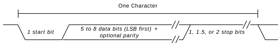
Figure 36 • UART Timing
