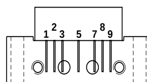
Fig.1 Simplified outline.
