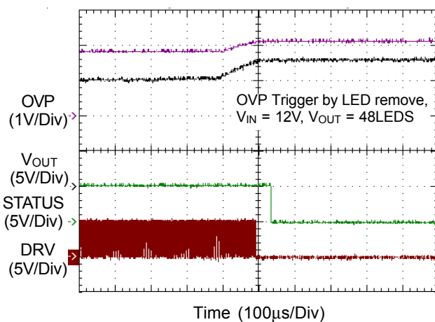
OVP Protection
