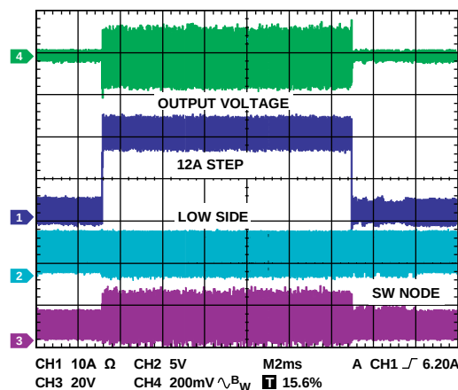
Figure 50. Load Transient Step—Forced PWM at Light Load, 12 A (See Figure 94 Application Circuit)
