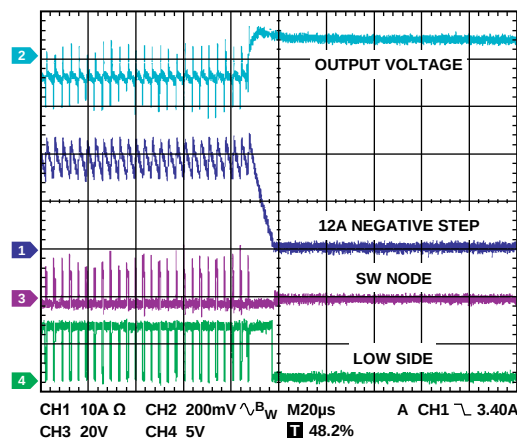
Figure 49. Negative Step During Heavy Load Transient Behavior—PSM Enabled, 12 A (See Figure 94 Application Circuit)
