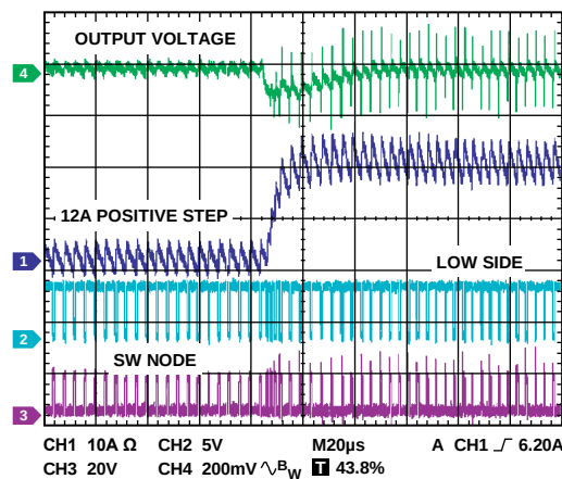
Figure 51. Positive Step During Heavy Load Transient Behavior—Forced PWM at Light Load, 12 A, V_{OUT} = 1.8 V (See Figure 94 Application Circuit)
