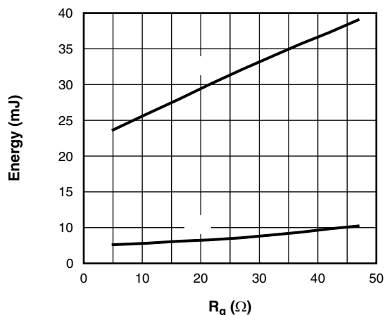
Fig. 11 - Typical IGBT Energy Loss vs. R_g T_J = 125^\circ\text{C} , I_C = 100\text{ A} , L = 500\text{ }\mu\text{H} , V_{CC} = 600\text{ V} , V_{GE} = 15\text{ V}
