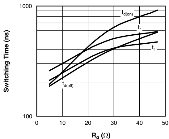
Fig. 12 - Typical IGBT Switching Time vs. R_g T_J = 125^\circ\text{C} , L = 500\text{ }\mu\text{H} , V_{CC} = 600\text{ V} , I_C = 100\text{ A} , V_{GE} = 15\text{ V}
