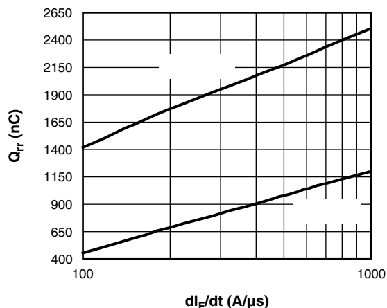
Fig. 15 - Typical Q_{rr} Diode vs. dI_F/dt V_R = 200\text{ V} , I_F = 50\text{ A}
