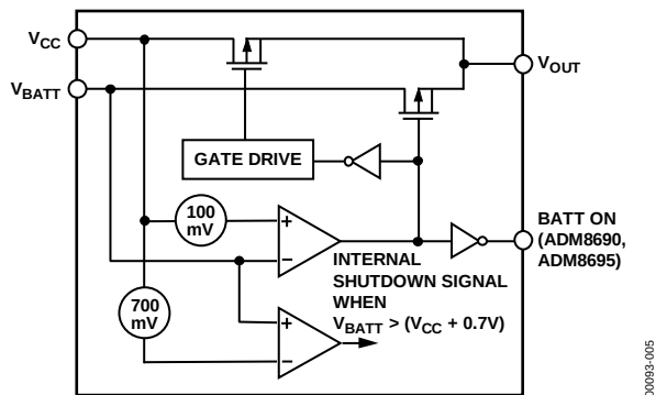
Figure 14. Battery Switchover Schematic
