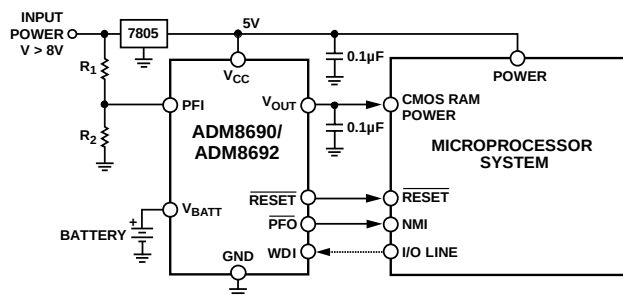
Figure 31. ADM8690/ADM8692 Typical Application Circuit B
