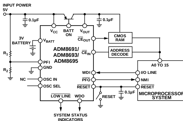
Figure 32. ADM8691/ADM8693/ADM8695 Typical Application
