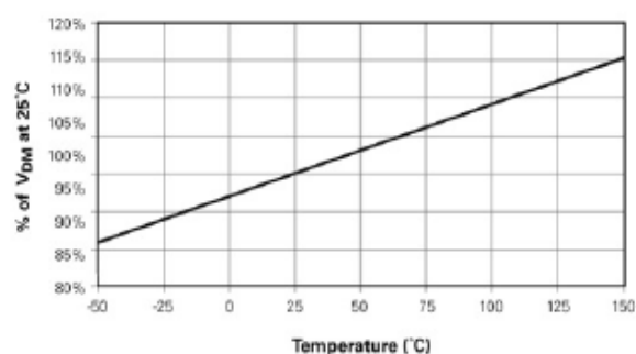
Figure SB3 - Off-state Voltage vs. Temperature
