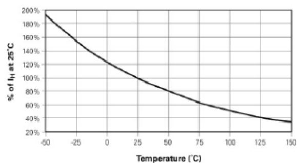
Figure SB5 - Hold Current vs. Temperature
