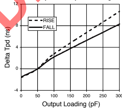
Delta Tpd vs Output Loading
