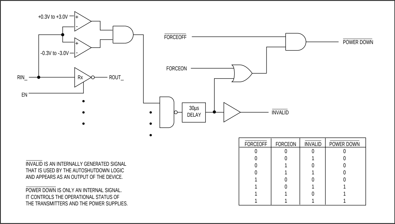
Figure 3. AutoShutdown Logic
