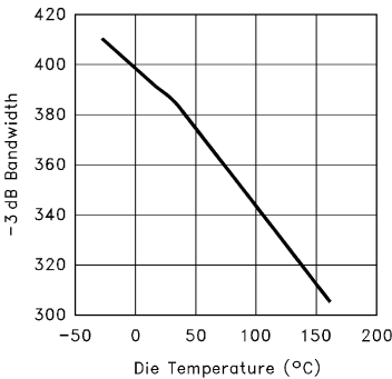
FIGURE 14. BANDWIDTH vs DIE TEMPERATURE
